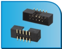
118-C SERIES BOX HEADER SMT 2.00mm(0.079 ")
