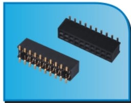
115-C SERIES P.C.B SOCKET SMT TYPE 1.27mm(0.050 ")
