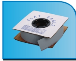
XYD020 FLAT CABLE 1.27mm COLOR:GREY SPECIFICATION:28AWG CONDUCTORS:10,14,16,20,26, 30,34,40,50,60,64 REEL:30.5M/76M
