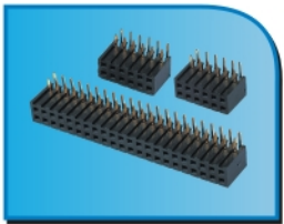
117-A SERIES FEMALE HEADER 2.0mm(0.079 ")
