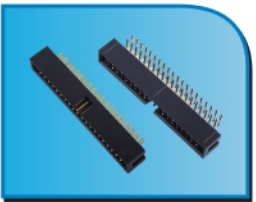
118-A SERIES BOX HEADER 2.54mm(0.100 ")
