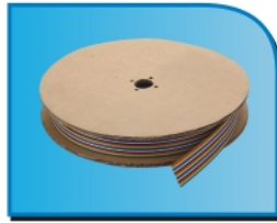
XYD021 COLOR FLAT CABLE SPECIFICATION:30AWG/28AWG/26AWG CONDUCTORS:10,14,16,20,26, 30,40,50,60,64 REEL:30.5M/76M
