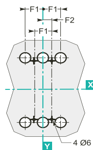
TEM7(E)-400/630 3P
